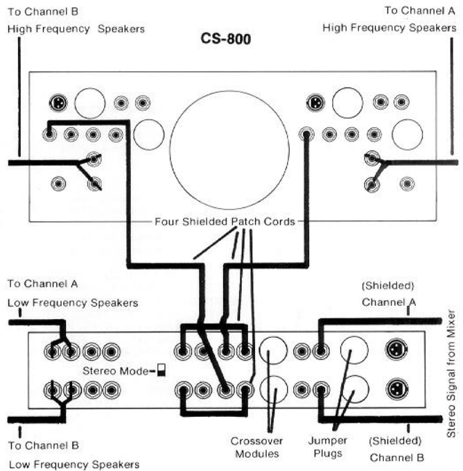
CS-1200 PATCH DIAGRAM 6 Biamp Operation Unbalanced High Z Inputs (Stereo Signal)
